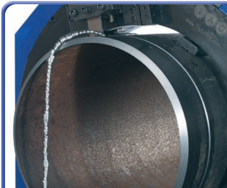
Pipe cutting
